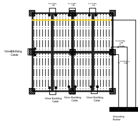
solar PV panels string 1 and 2 for solar inverter No.2
