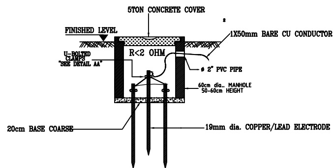
EARTHING MANHOLE DETAIL
