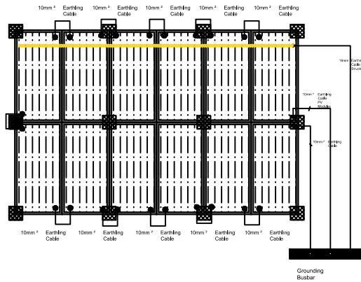
solar PV panels string 1 for solar inverter No.1
