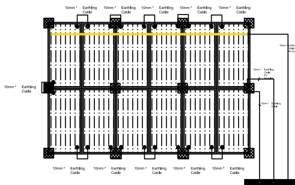
solar PV panels string 2 for solar inverter No.1
