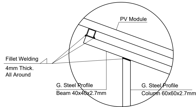
Detail 2 Scale 1:10
