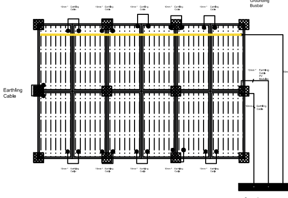
solar PV panels string 2 for solar inverter No.2
