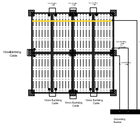
Grounding Bonding Busbar
