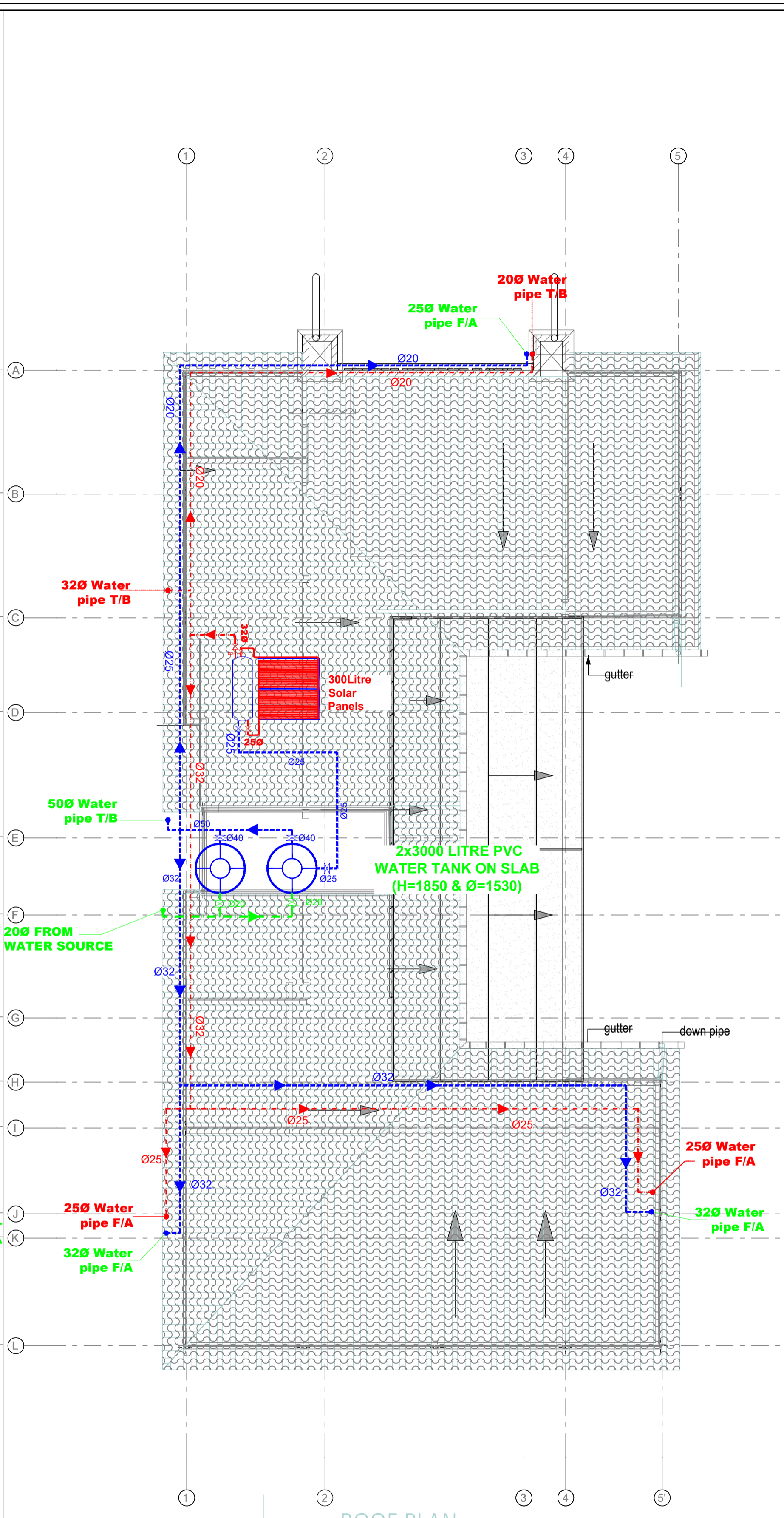
ROOF PLAN
