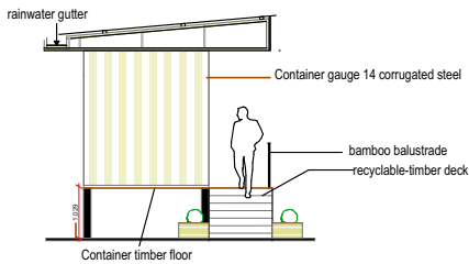
ELEVATION D SCALE 1:100
