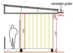
ELEVATION B SCALE 1:100
