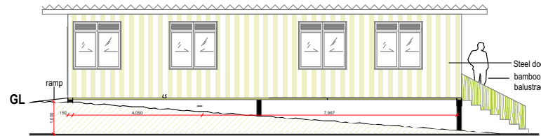
ELEVATION A SCALE 1:100
