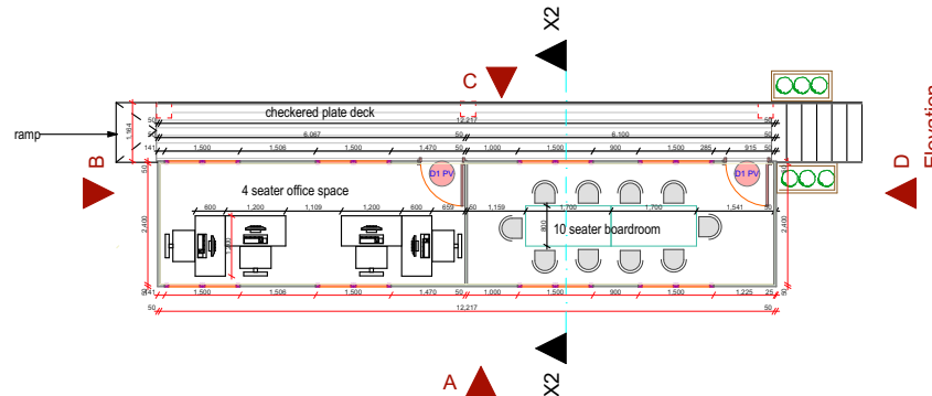
FLOOR PLAN SCALE 1:100
