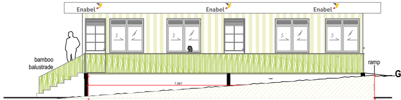
ELEVATION C SCALE 1:100
