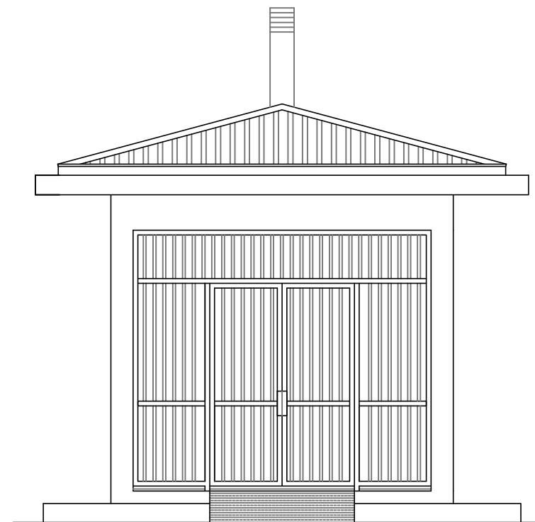
ELEVATION 1-1 INCINERATOR HOUSE Scale 1: 100
