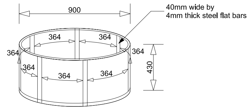
Cylindrical steel pot stabilizer for 250 litre capacity cooking pot made from 40mm wide by 4mm thick flat steel bars
