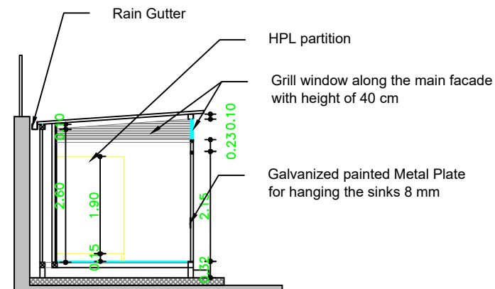
Section 2-2
