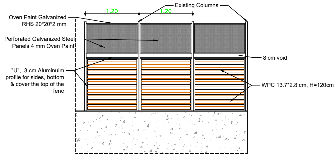
External Fence Detail Scale 1:50
