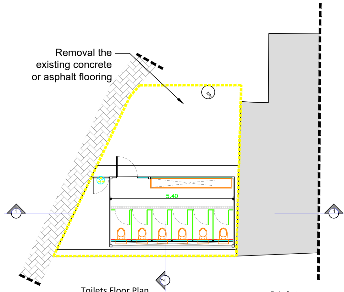
Toilets Floor Plan Scale 1:100
