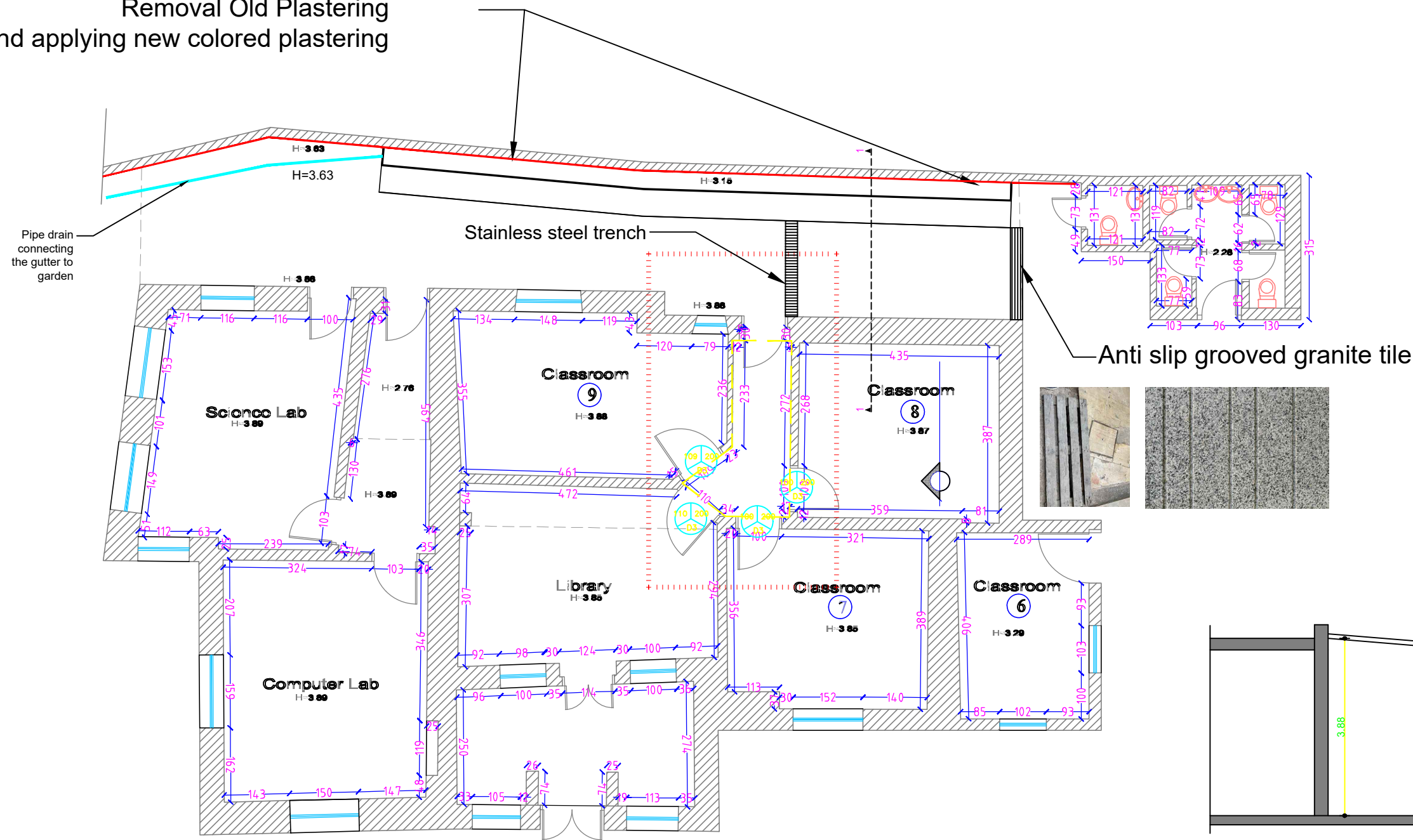
Ground Floor Plan- scale 1:100 Building 3
