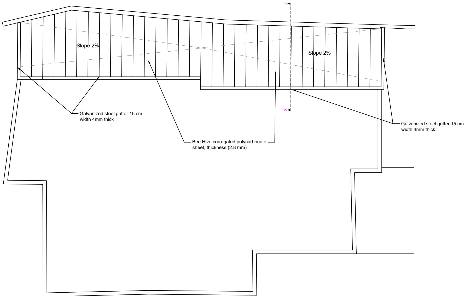
Ground Floor Plan- scale 1:100 Building 3
