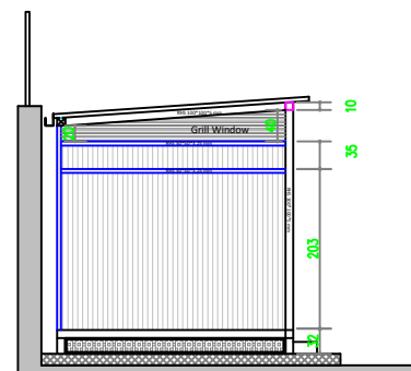
Side elevations
