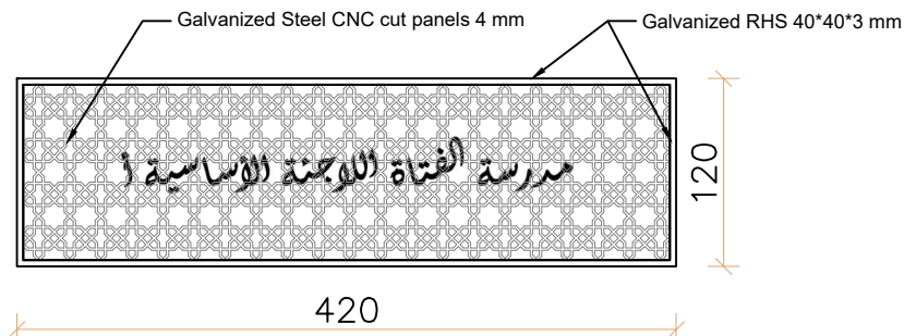
CNC Cut Scale 1:50
