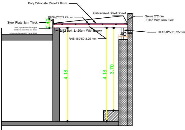
Section 1-1
