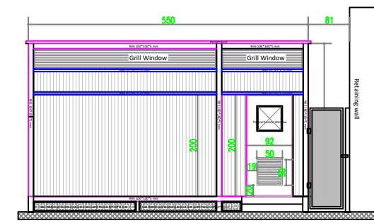
Main elevation
