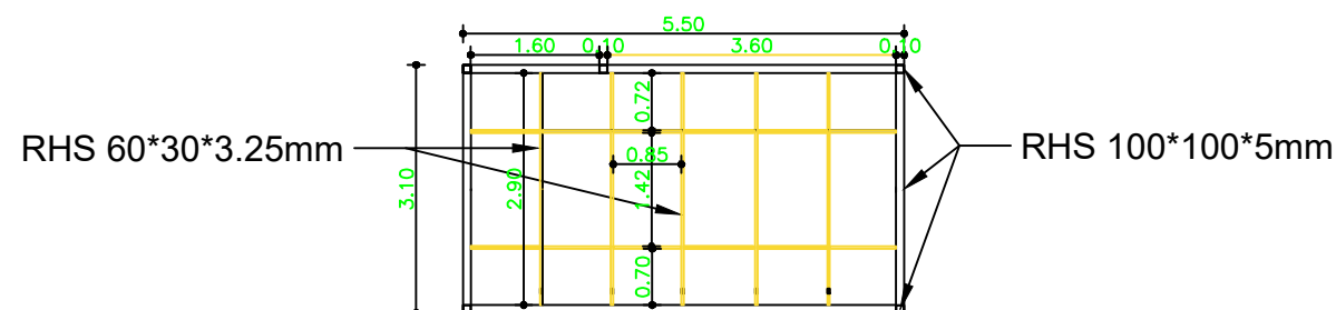
Roof Steel Detail
