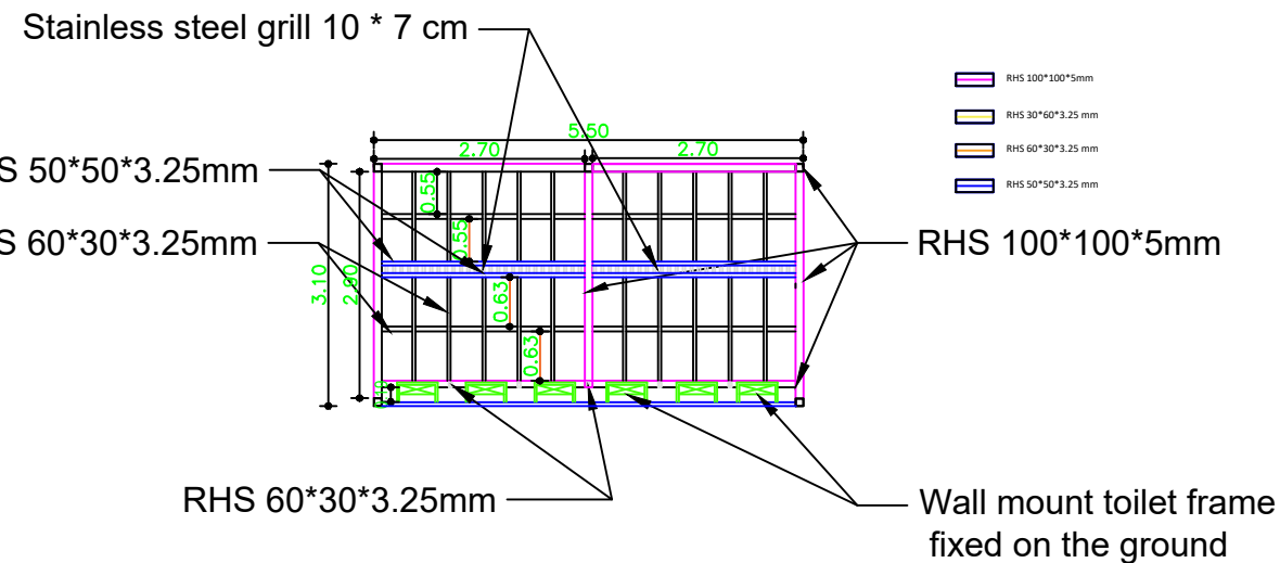
Steel Floor Platform Detail
