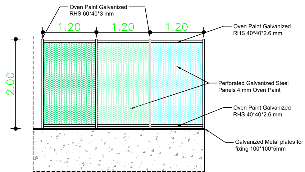
External Fence Detail Scale 1:50
