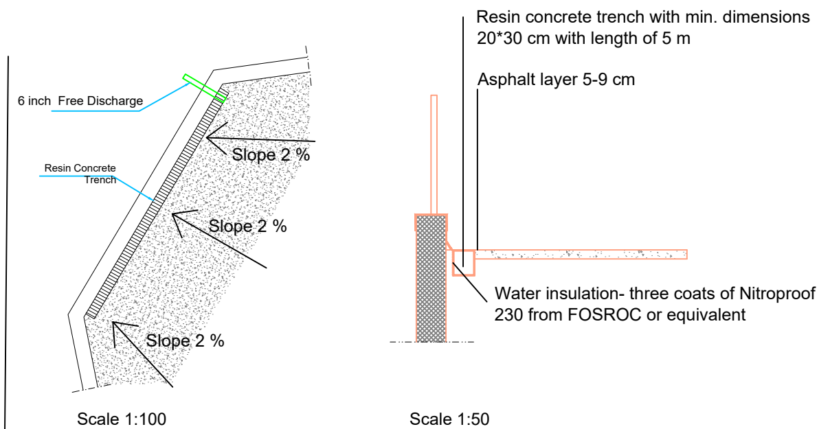
D3: Drainage trenches & adjusting slope
