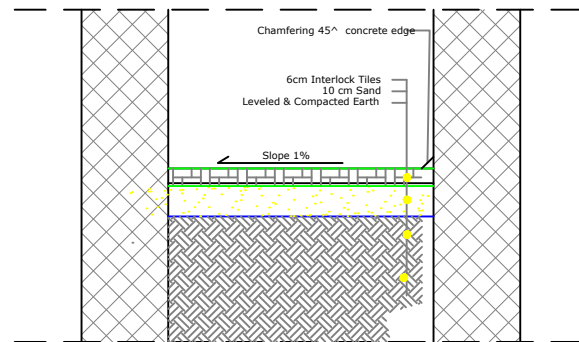
Detailed Sec. 1-1 Scale 1:25
