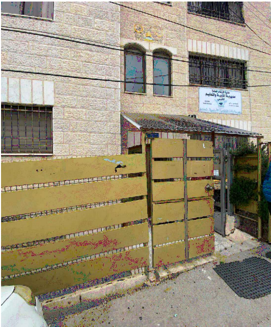
D2: Metal Fence Detail- Align the street The same as in the main elevation of school Galvanized steel 3 mm thick
