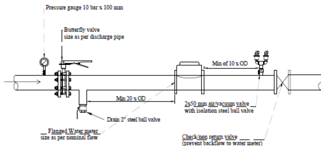
Figure 4. Example for installation of analogical flow-meter.
