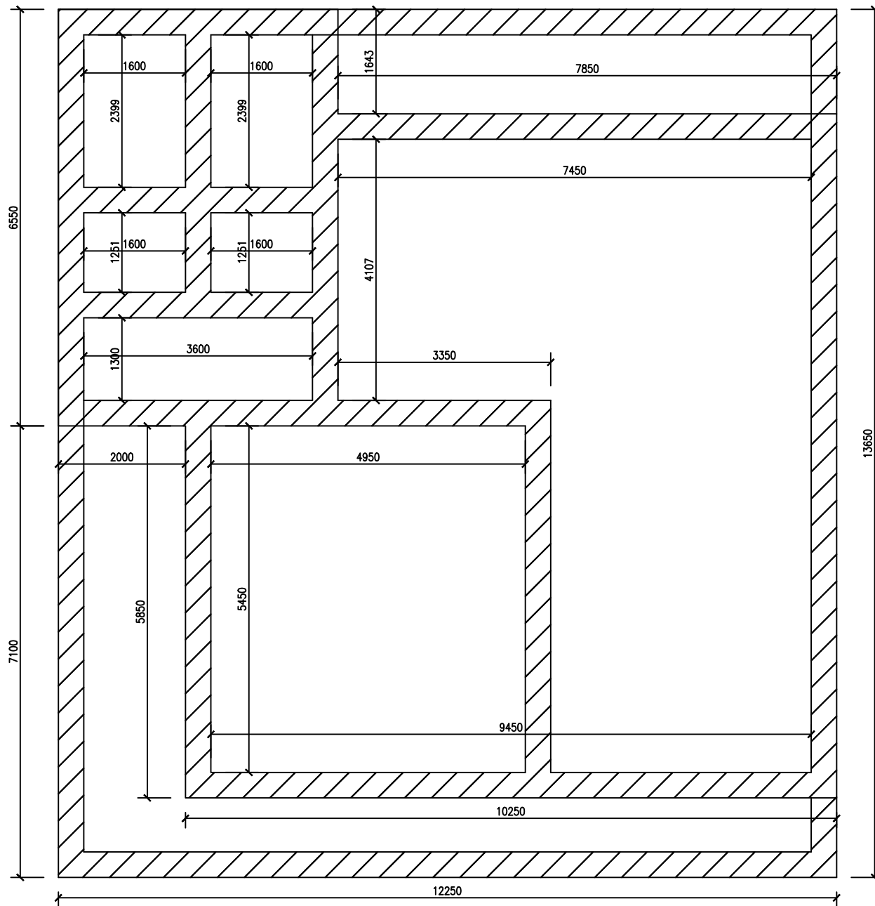
Foundation Plan
