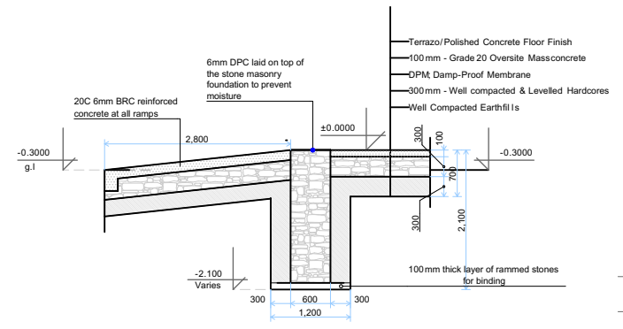
SECTION 3
