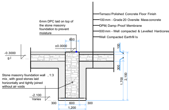
SECTION 2-2
