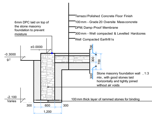
SECTION -1
