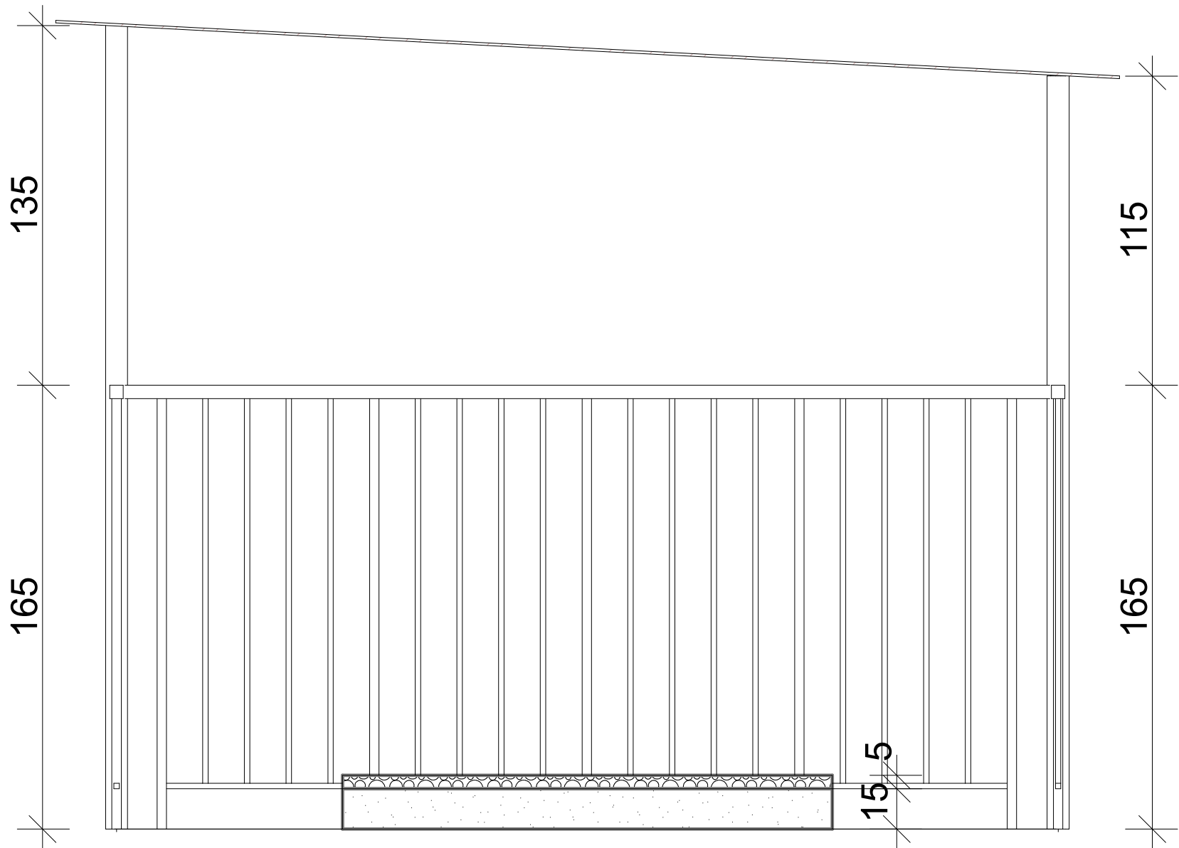
FACADE TRANSVERSALE
