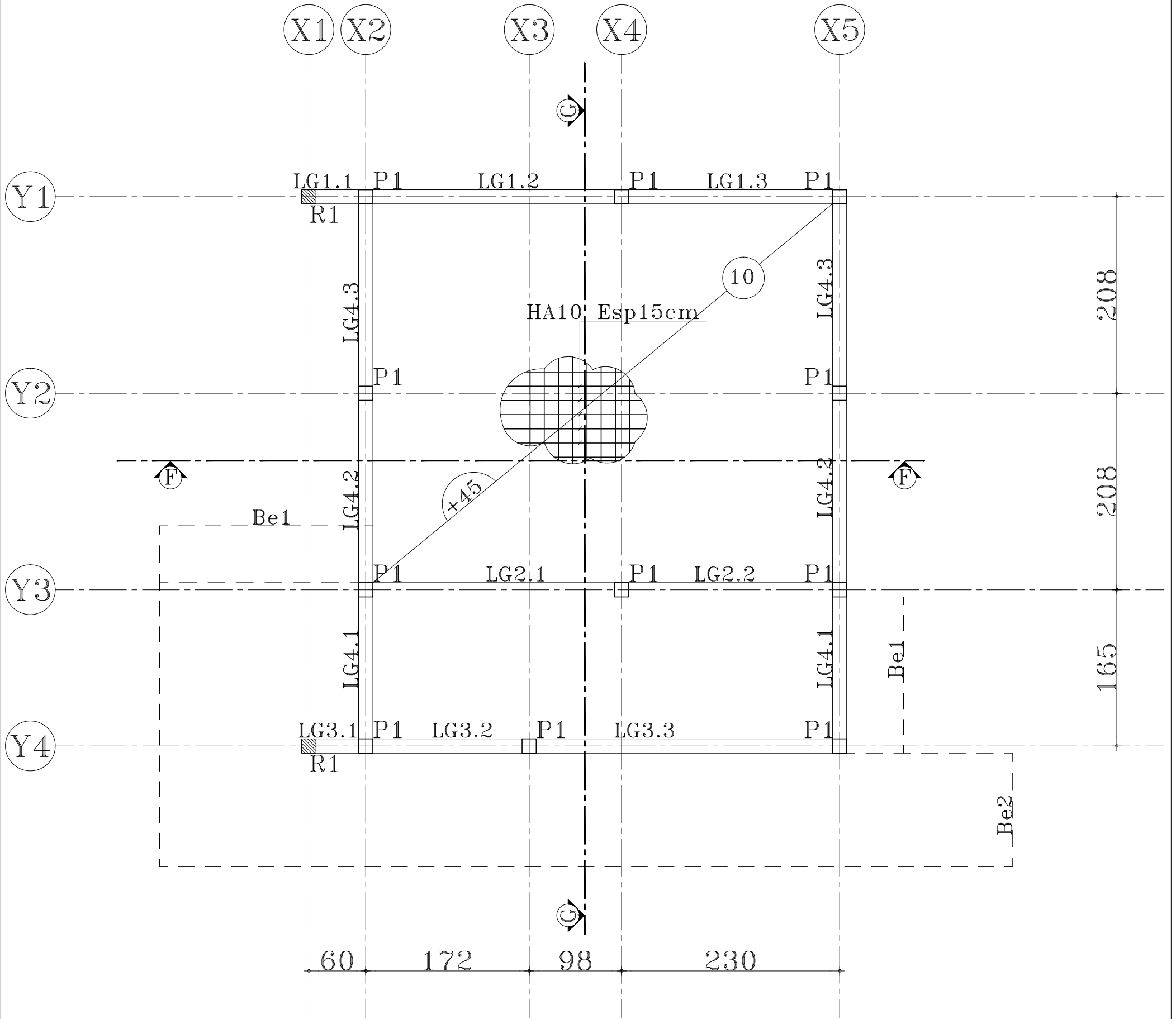
ENSEMBLE LONGRINES DALLAGE COFFRAGE +0.45m/TN
