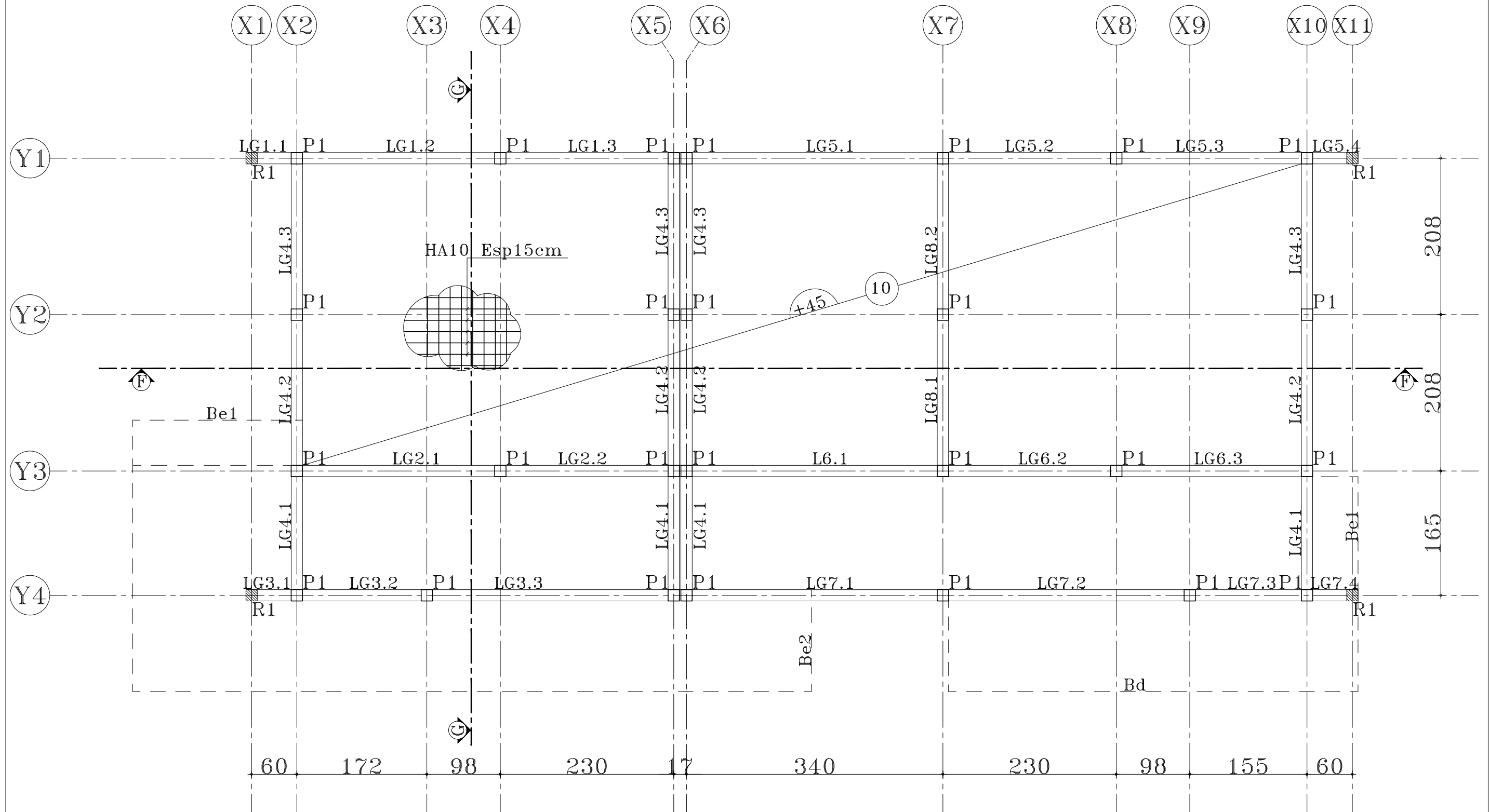
ENSEMBLE LONGRINES DALLAGE COFFRAGE +0.45m/TN
