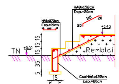
BECHE COUPE DETAIL 2-2 (Ferrillage)
