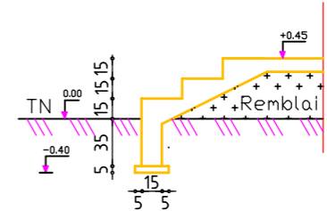
BECHE COUPE DETAIL 3-3 (Coffrage)
