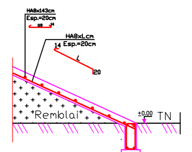
BECHE COUPE DETAIL 2-2 (Ferrillage)
