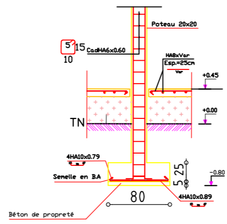
COUPE DETAIL 4-4
