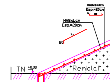
BECHE COUPE DETAIL 2-2 (Ferrillage)
