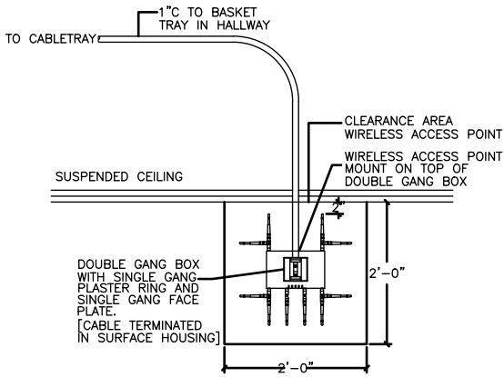
AP NETWORK ANTENNA MOUNTED ON WALL
