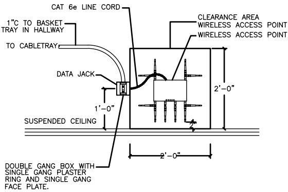
AP NETWORK ANTENNA MOUNTED ABOVE CEILING
