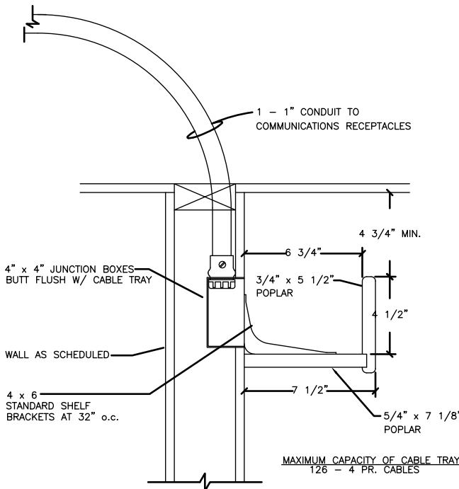
TELECOMMUNICATIONS TYPICAL CABLE TRAY BELOW CEILING
