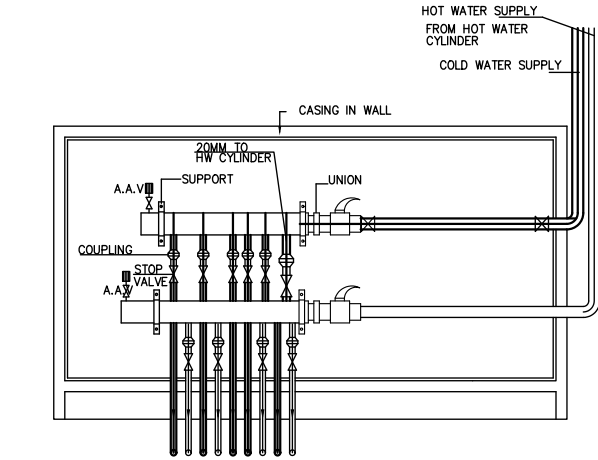
WATER CABINETS DETAIL
