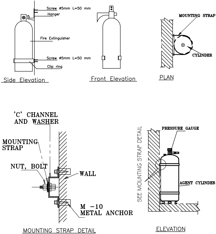
MOUNTING STRAP DETAIL
