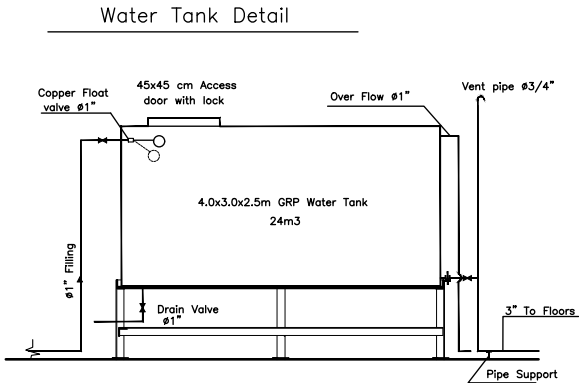
Water Tank Detail
