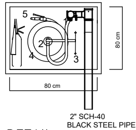
FIRE HOSE CABINET DETAIL
