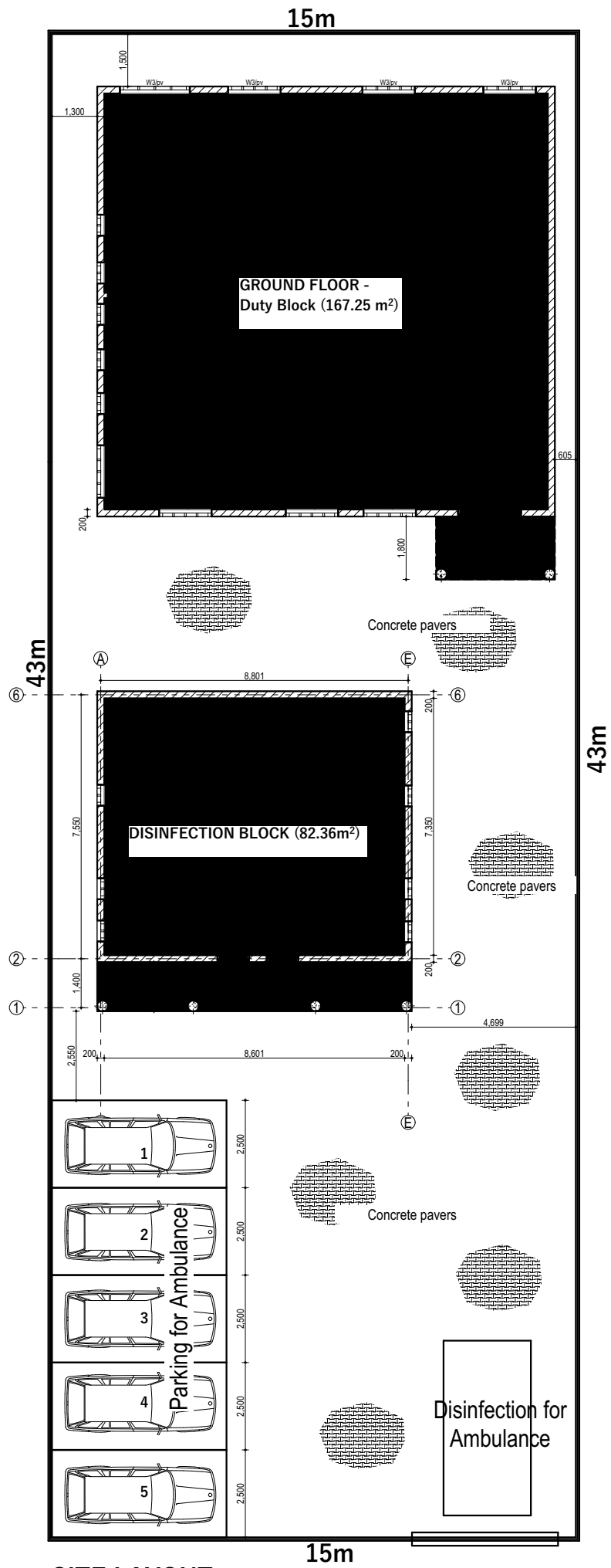
SITE LAYOUT, Arau RRH
